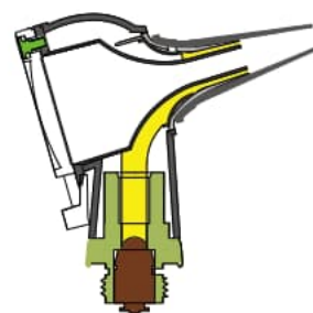
Fiber optic illumination
